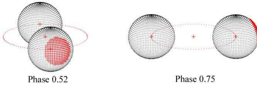
Figure 5. Binary Maker 3 representation of the system – at phases 0.52 and 0.75.
