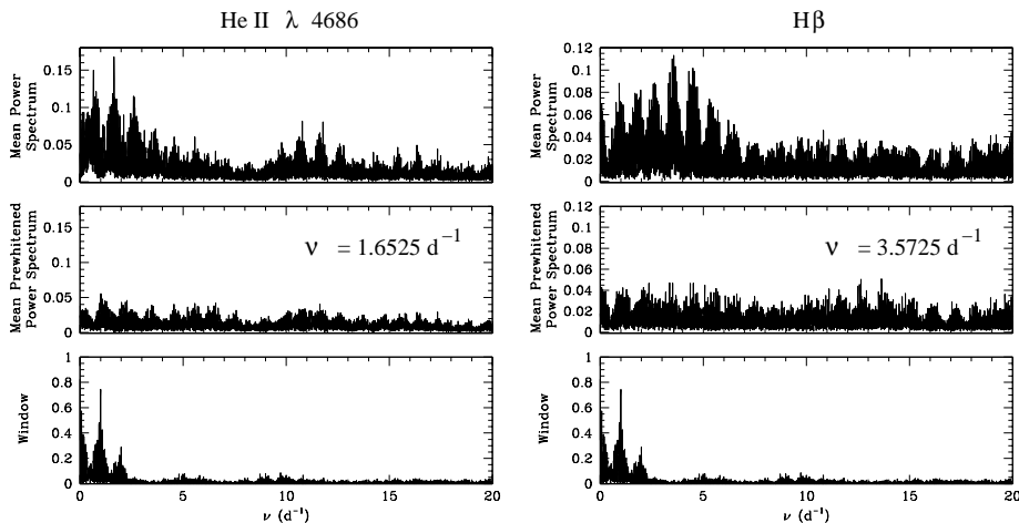
Figure 1. Fourier analysis of He II \lambda 4686 between 4682 and 4685 \text{\AA} ( left part ) and H \beta between 4857 and 4860 \text{\AA} ( right part ) in the case of HD 13268. Upper panels: mean power spectrum over the specified wavelength domain. Middle panels: prewhitened power spectrum using the specified frequency corresponding to the highest peak in the upper panel. Significant residual power is still present, but a much better sampling of higher frequencies is requested in order to determine accurately the variability time scales. Lower panels: spectral window related to the data sampling.
