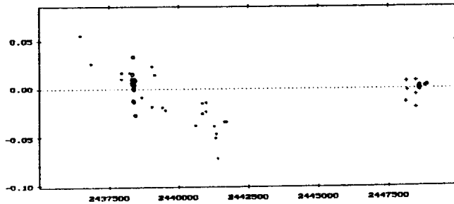
Figure 2: (O-C) Diagram for V432 Per computed with respect to the ephemeris (1). ● represents photoelectric, ○ photographic, + visual observations and ■ photographic plate minima.
